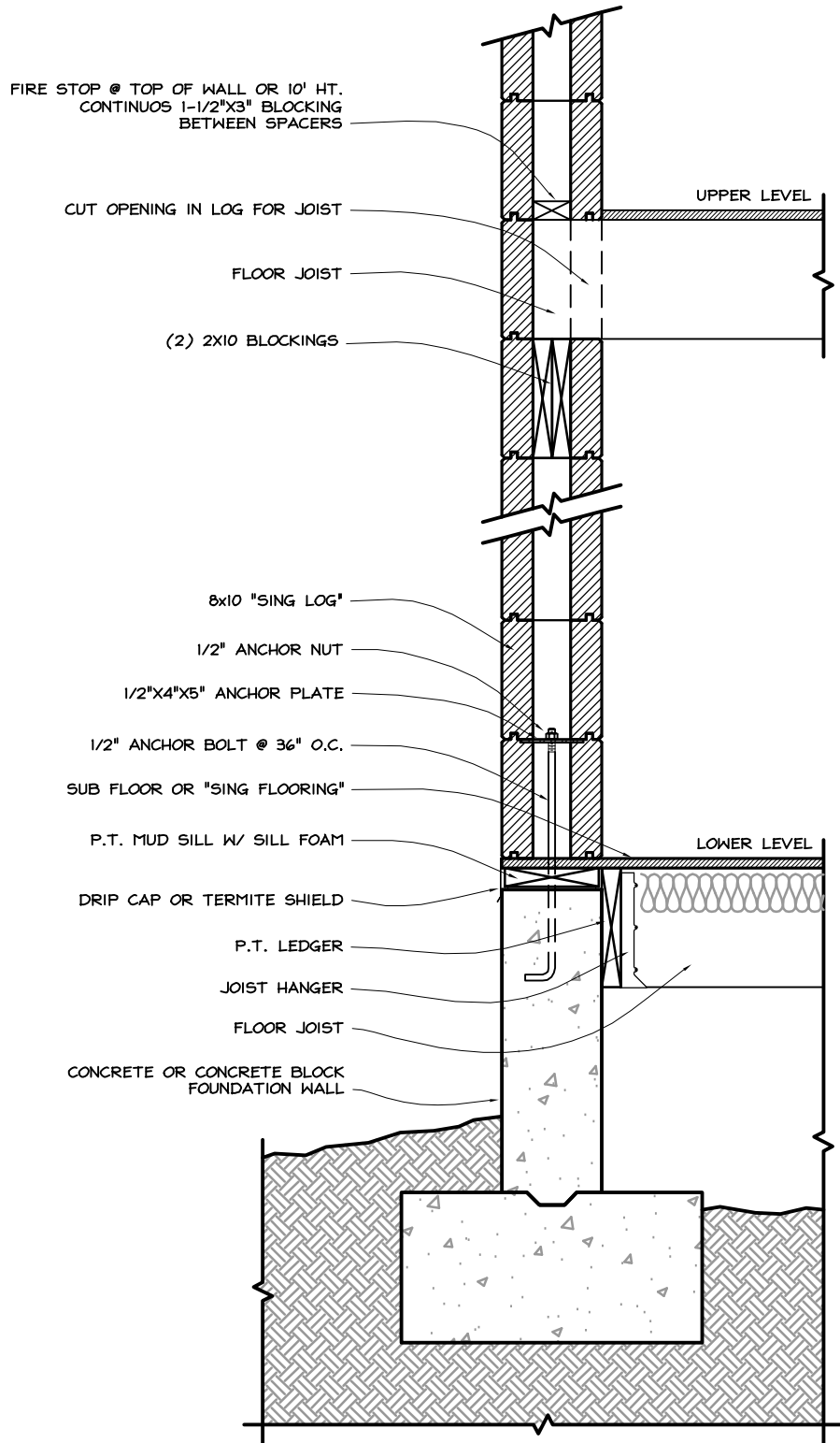
1 TYPICAL WALL SECTION, OPTION 1 D-03
